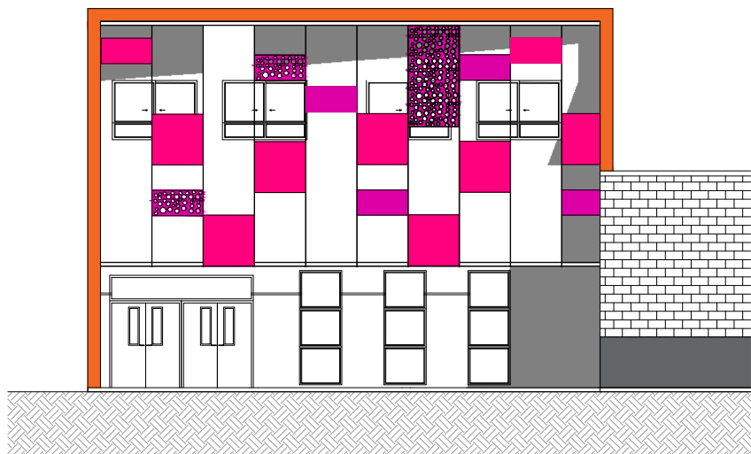
CHADA PRINCIPAL
